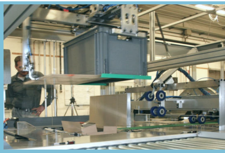
VARY-TOTES OPENING AND ITEMS DROPPING
